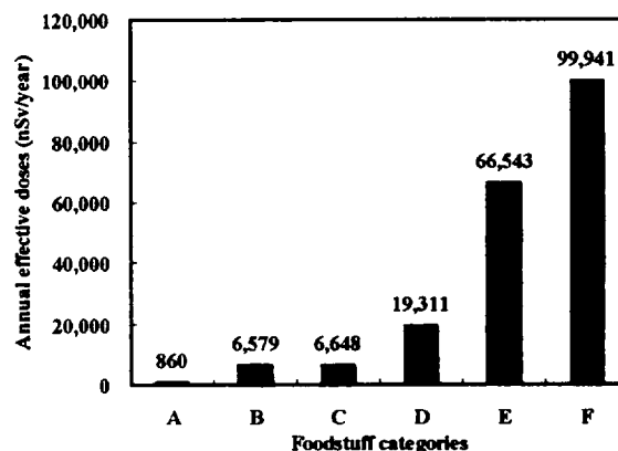
Fig. 1. Distribution of total annual effective dose according to foodstuff categories (A: forest products, B: marine products, C: processed foods, D: livestock products, E: agricultural products, F: all foodstuffs).
