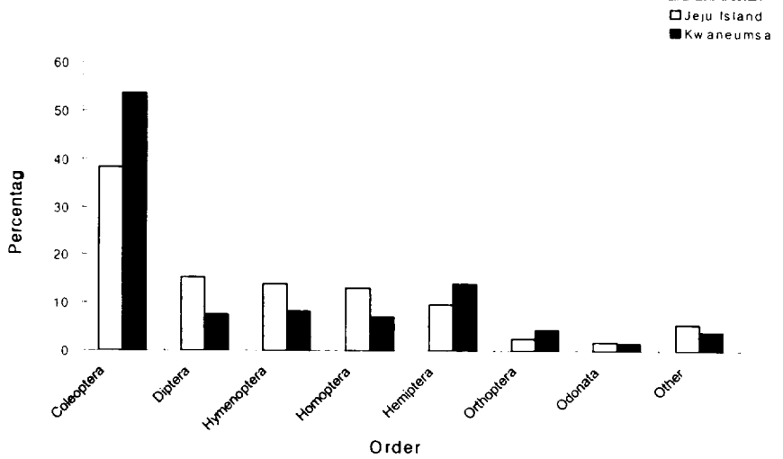
Figure 1. Percentage composition of species number for each order.
