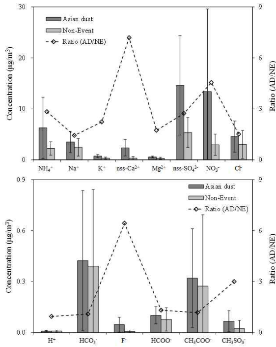
Figure 18. Comparison of concentrations and their ratios of ionic species in PM_{10} aerosols during Asian dust (AD) and non-event (NE) days.
