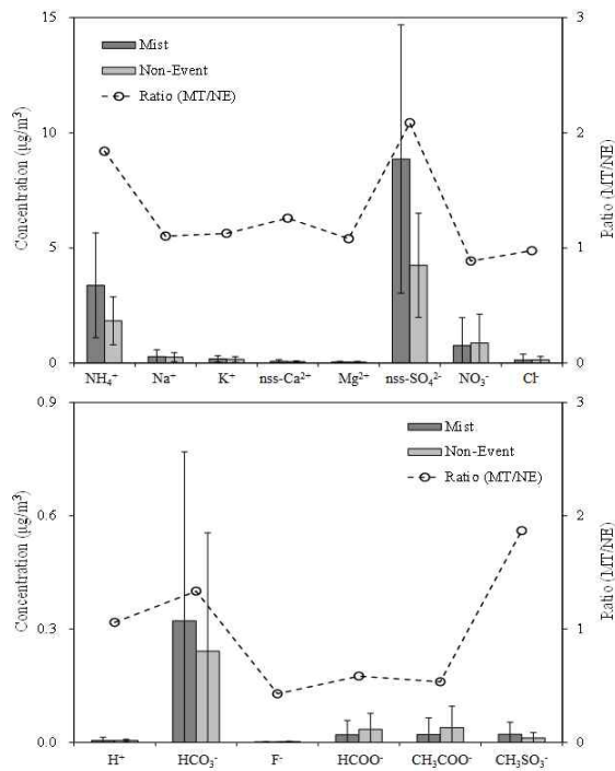
Figure 36. Comparison of concentrations and their ratios of ionic species in PM_{2.5} aerosols during mist (MT) and non-event (NE) days.
