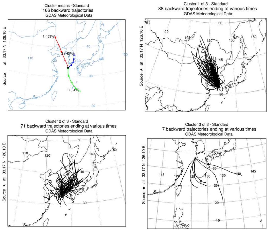
Figure 16. Clustered back trajectories of air masses at Gosan site.
