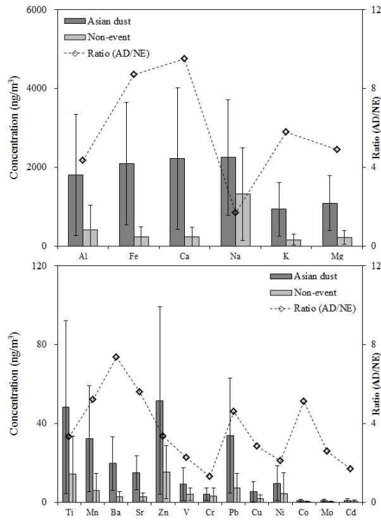
Figure 22. Comparison of concentrations and their ratios of elemental species in PM_{10} aerosols during Asian dust (AD) and non-event (NE) days.
