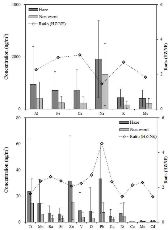
Figure 30. Comparison of concentrations and their ratios of elemental species in PM_{10} aerosols during haze (HZ) and non-event (NE) days.
