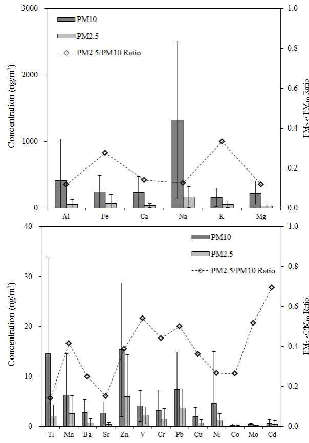
Figure 14. Comparison of concentrations and their ratios of elemental species in PM 10 and PM 2.5 aerosols.
