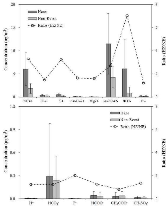
Figure 27. Comparison of concentrations and their ratios of ionic species in PM_{2.5} aerosols during haze (HZ) and non-event (NE) days.
