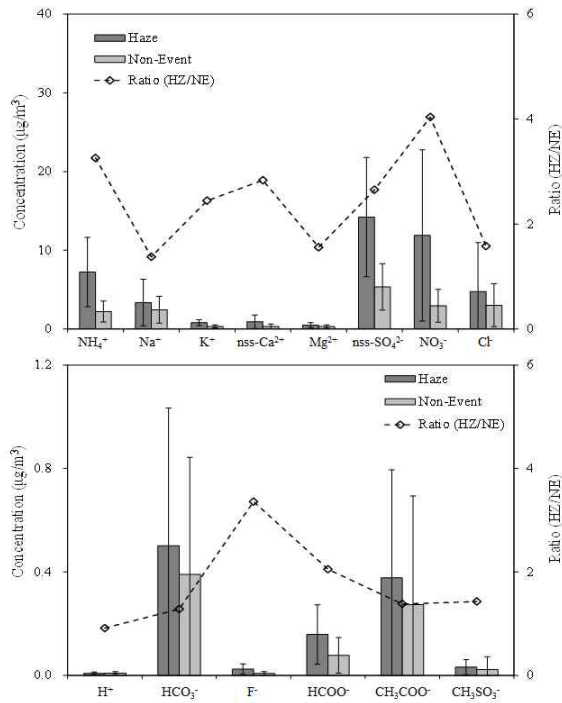
Figure 26. Comparison of concentrations and their ratios of ionic species in PM_{10} aerosols during haze (HZ) and non-event (NE) days.
