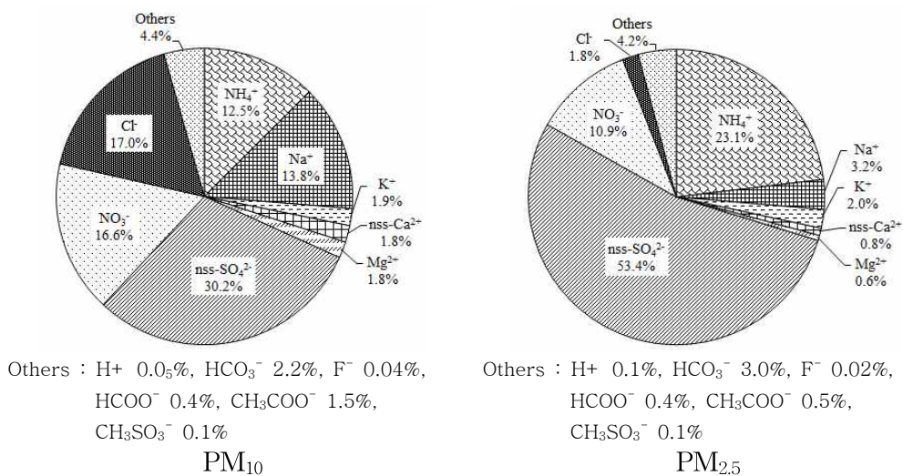
Figure 13. Composition ratios of ionic species in PM_{10} and PM_{2.5} aerosols.
