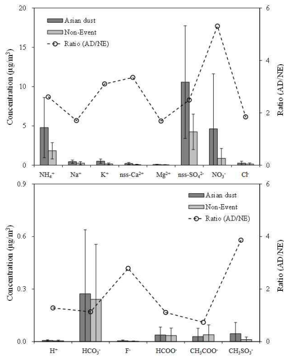
Figure 19. Comparison of concentrations and their ratios of ionic species in PM_{2.5} aerosols during Asian dust (AD) and non-event (NE) days.
