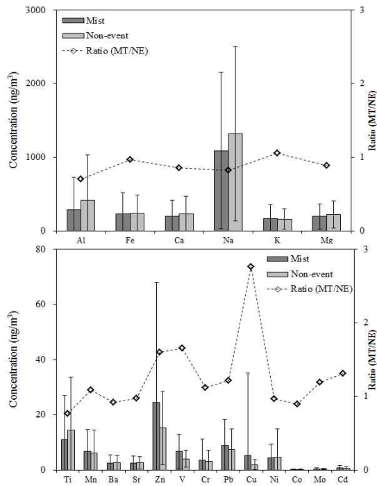
Figure 39. Comparison of concentrations and their ratios of elemental species in PM_{10} aerosols during mist (MT) and non-event (NE) days.
