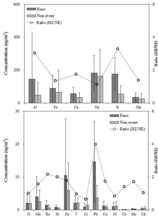
Figure 31. Comparison of concentrations and their ratios of elemental species in PM_{2.5} aerosols during haze (HZ) and non-event (NE) days.
