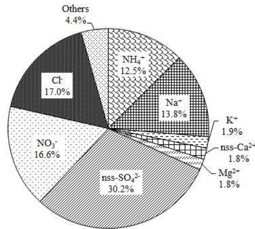
Figure 4. Comparison of ionic concentrations in \text{PM}_{10} aerosols.
