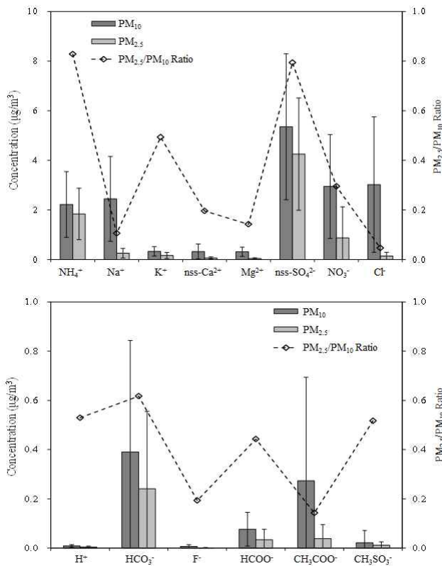
Figure 12. Comparison of concentrations and their ratios of ionic species in PM_{10} and PM_{2.5} aerosols.
