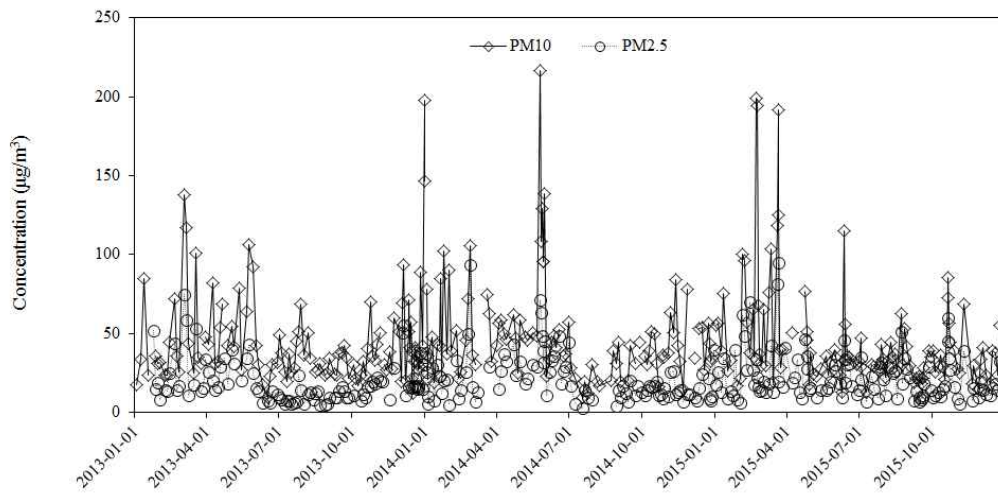
Figure 1. Variations of PM 10 , and PM 2.5 mass concentrations at Gosan site during the study
