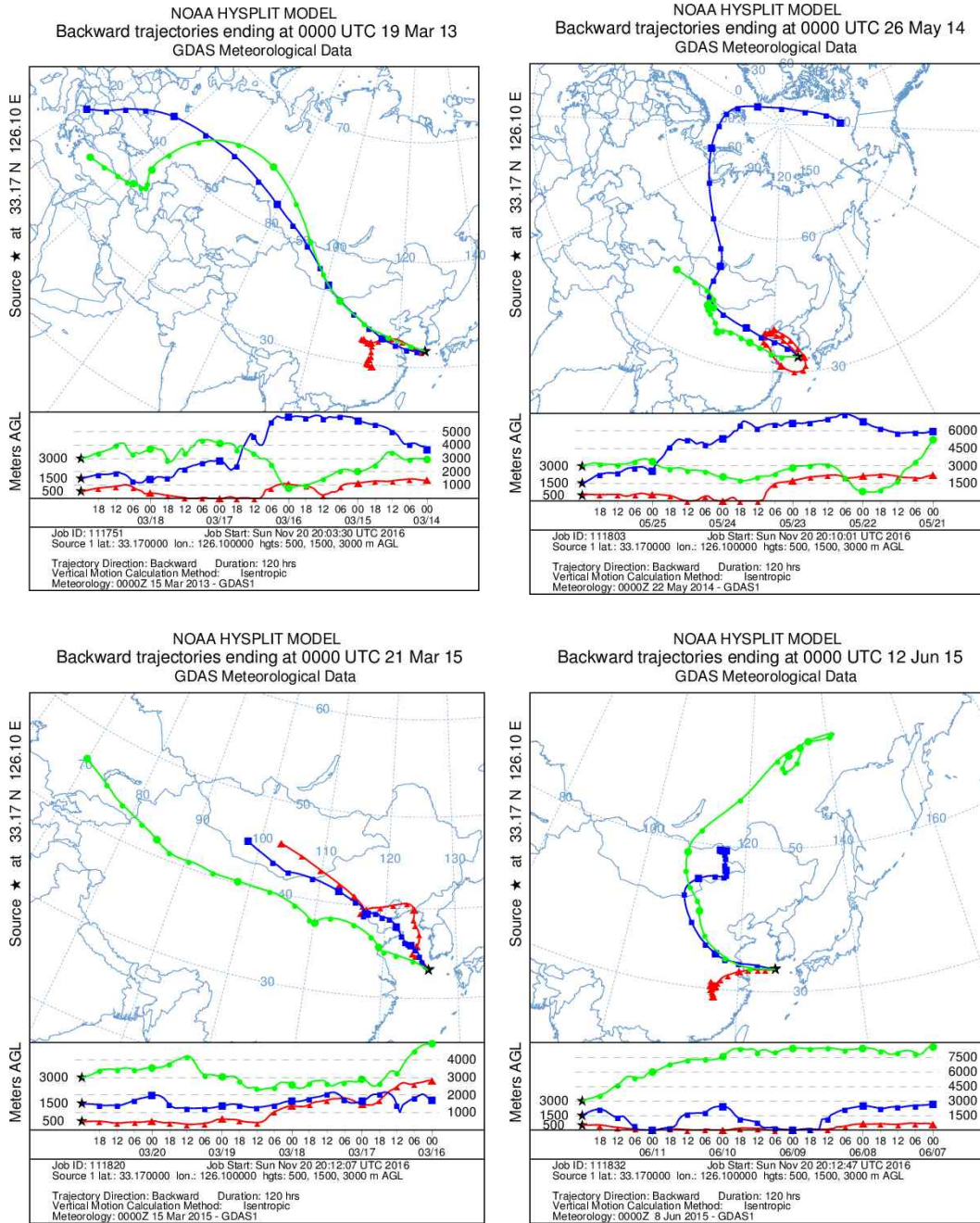
Figure 17. 5-Day back trajectories for the Asian dust days on Mar 19th, 2013, May 26th, 2014, Mar 21st, 2015 and Jun 12th, 2015 at Gosan site.
