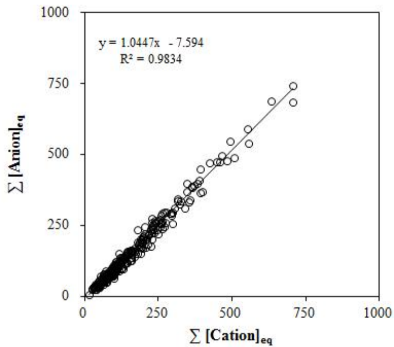
Figure 3. Correlations of \Sigma[\text{Cation}]_{\text{eq}} versus \Sigma[\text{Anion}]_{\text{eq}} for the analytical data of \text{PM}_{2.5} aerosols at Gosan site.
