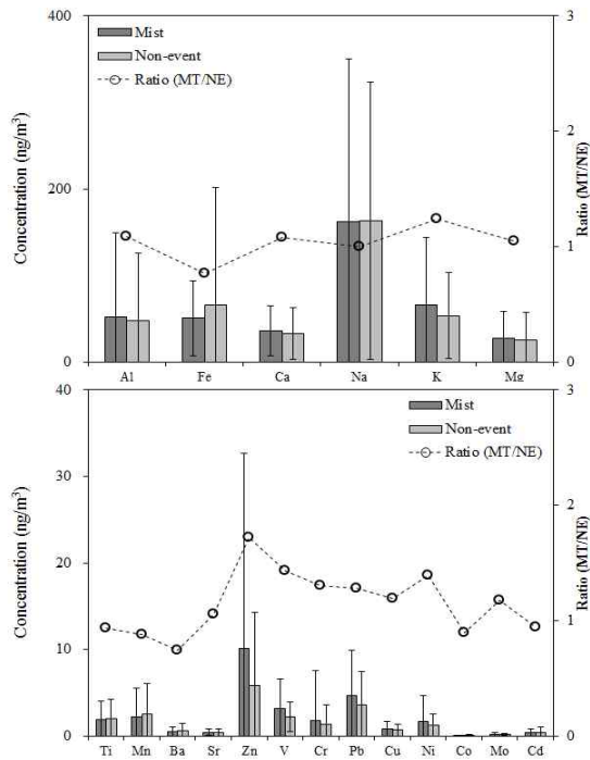
Figure 40. Comparison of concentrations and their ratios of elemental species in PM_{2.5} aerosols during mist (MT) and non-event (NE) days.
