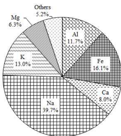
Figure 10. Comparison of elemental concentrations in PM 2.5 aerosols.
