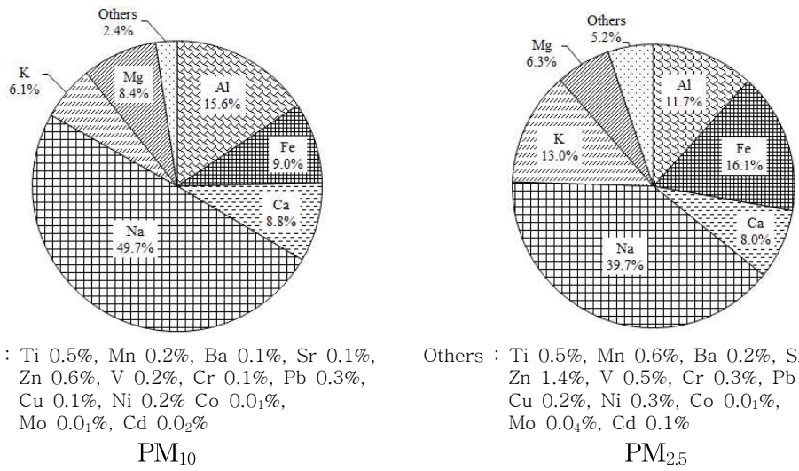
Figure 15. Composition ratio of elemental species in PM 10 and PM 2.5 aerosols.
