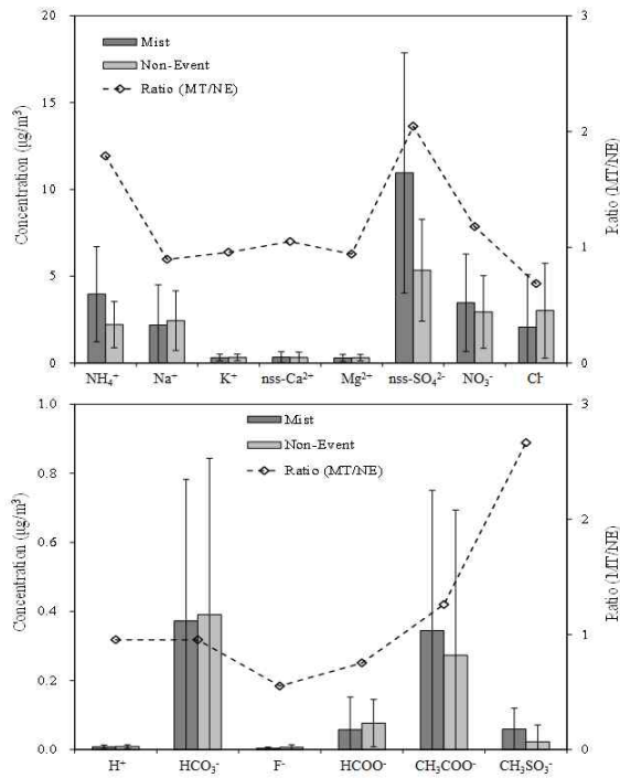
Figure 35. Comparison of concentrations and their ratios of ionic species in PM_{10} aerosols during mist (MT) and non-event (NE) days.
