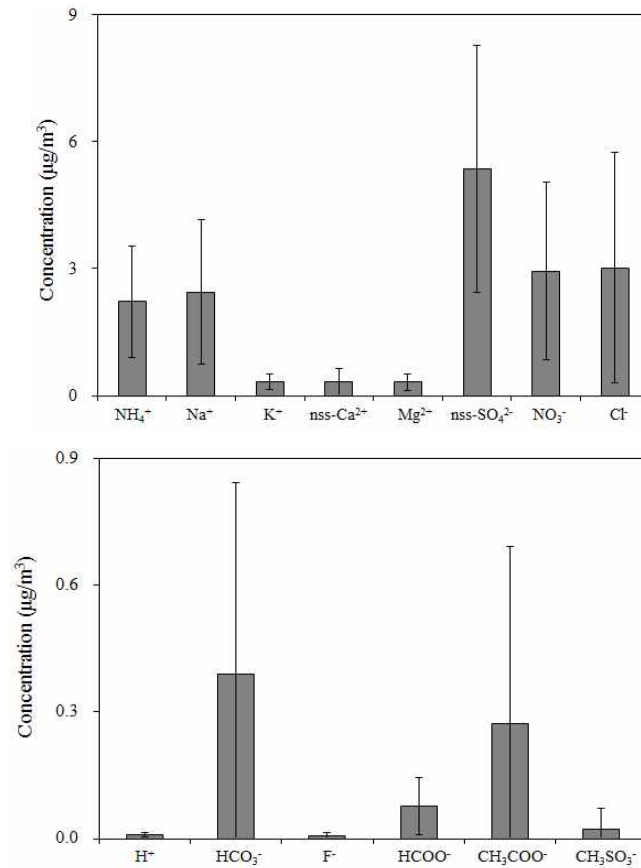
Figure 4. Comparison of ionic concentrations in \text{PM}_{10} aerosols.
