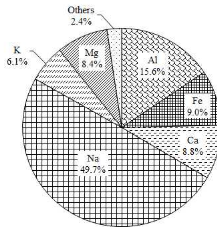
Figure 6. Comparison of elemental concentrations in PM 10 aerosols.
