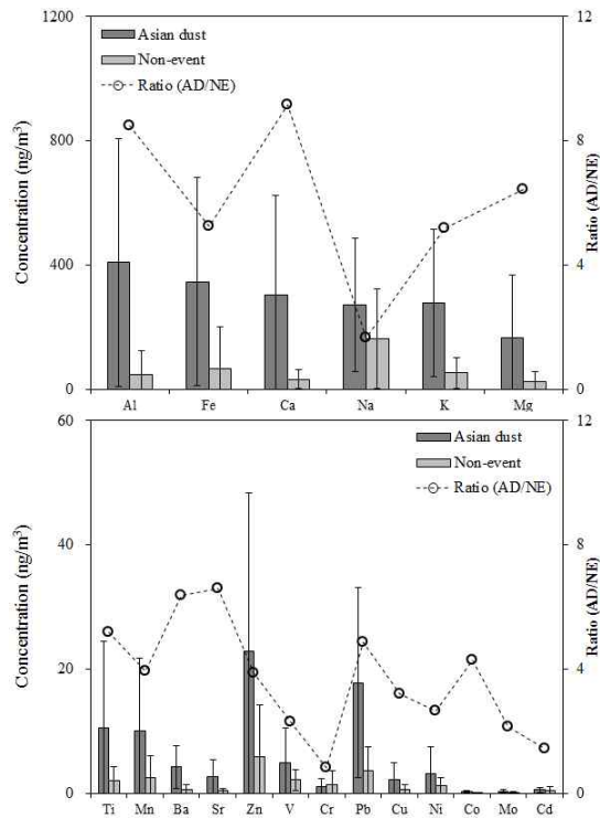
Figure 23. Comparison of concentrations and their ratios of elemental species in PM_{2.5} aerosols during Asian dust (AD) and non-event (NE) days.
