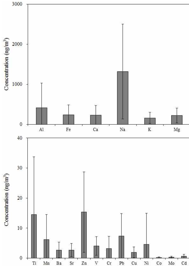
Figure 6. Comparison of elemental concentrations in PM 10 aerosols.
