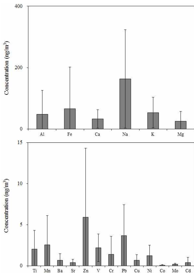
Figure 10. Comparison of elemental concentrations in PM 2.5 aerosols.
