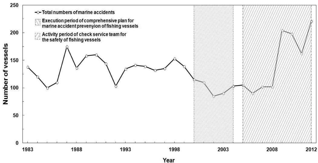
Fig. 3 A trend of total number of the marine accidents occurring in the sea around Jeju island and the execution period of comprehensive plan for marine accident prevention of fishing vessels(1983~2012).
