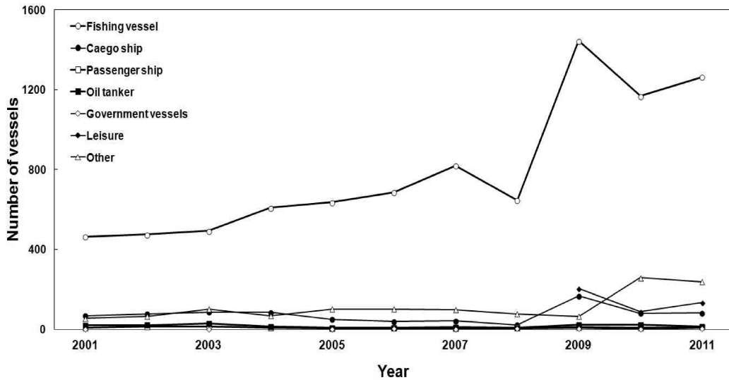
Fig 2 Variations of marine accidents depending on the type of vessels in the sea around Korea (2001~2011).
