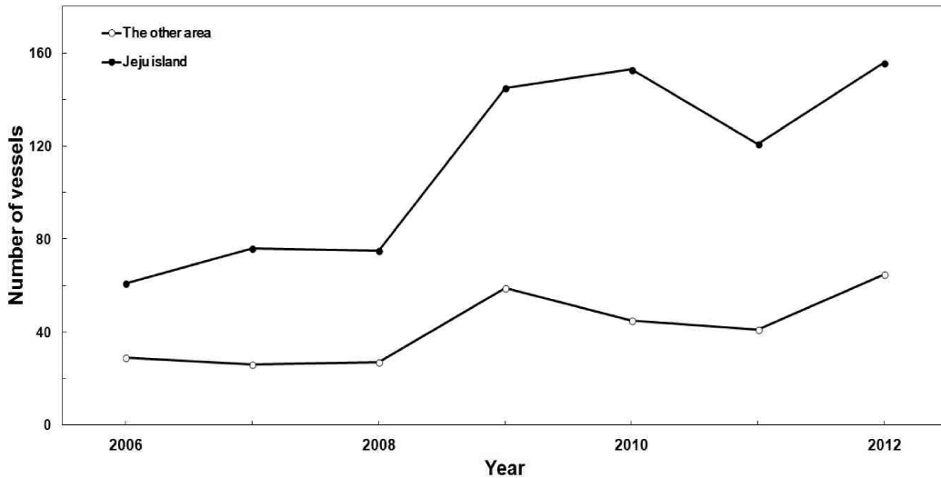
Fig. 4 Variations of marine accidents depending on the ports of registry in the sea around Jeju island(2006~2012).
