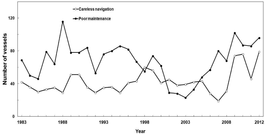
Fig. 9 Comparison between careless navigation and poor maintenance on the marine accidents occurring in the sea around Jeju island (1983~2012).
