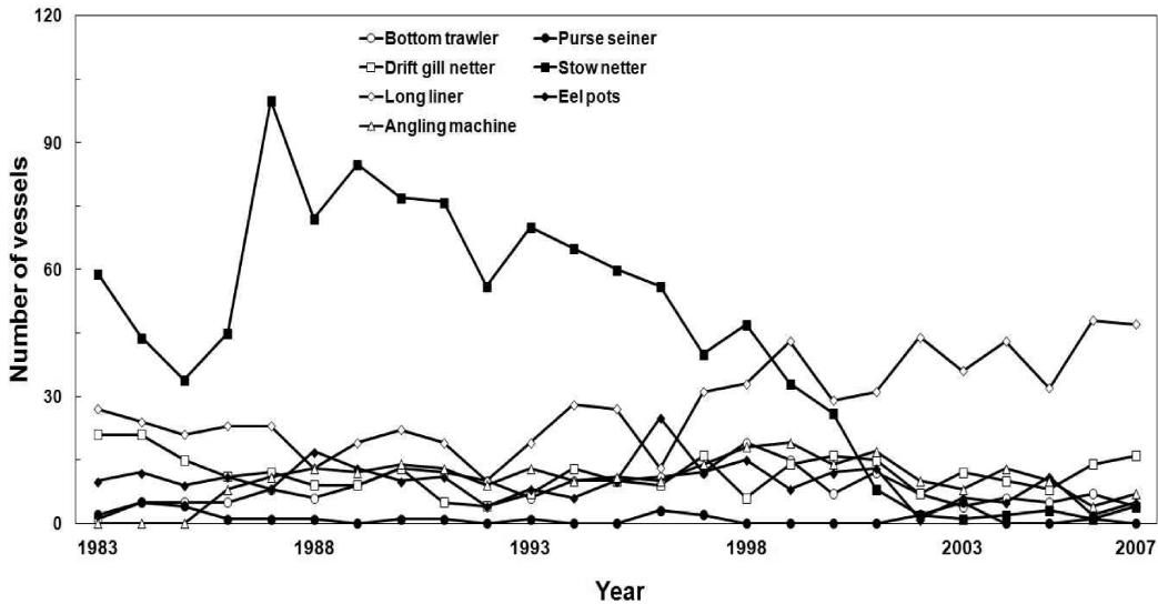
Fig. 8 Variations of marine accident depending on the fishing methods in the sea around Jeju island(1983~2007).
