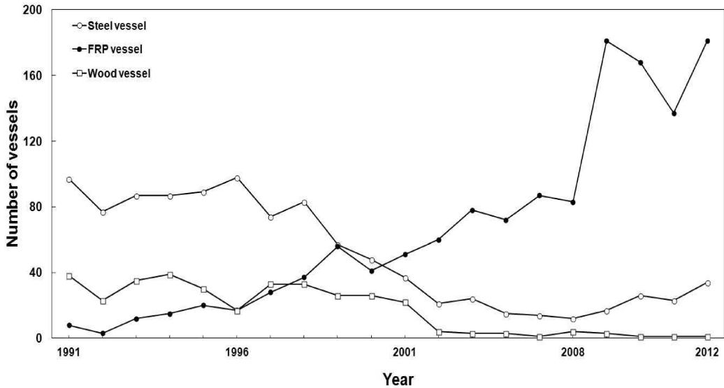
Fig. 6 Variations of marine accidents depending on the material of vessels in the sea around Jeju island(1991~2012).
