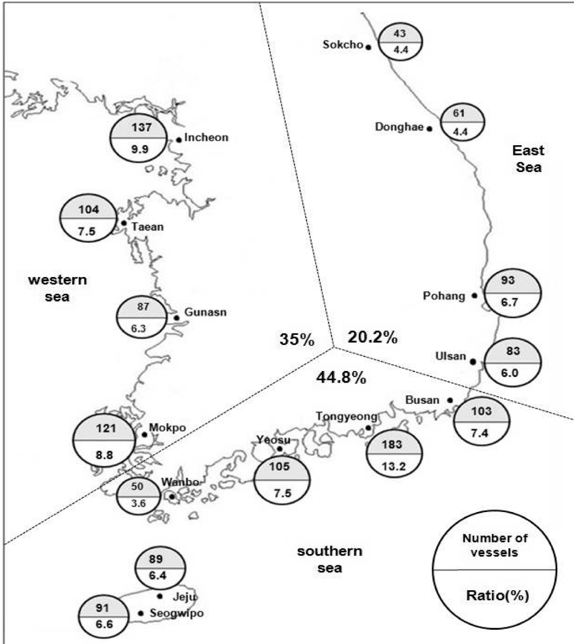
Fig. 1 The current numbers and its ratios of marine accidents occurring in the Each region of whole seas around Korea.(2006~2012).
