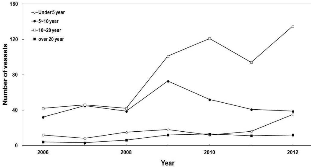
Fig. 7 Variations of marine accidents depending on the age of the vessels in the sea around Jeju island(2006~2012).
