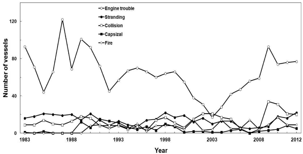
Fig. 10 Variations of marine accidents depending on the occurrence factors in the sea around Jeju island(1983~2012).
