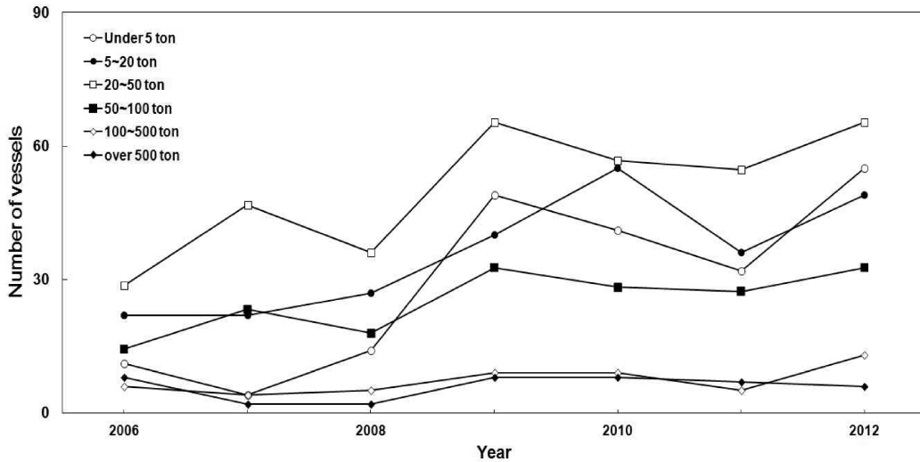
Fig. 5 Variations of marine accident depending on the tonnage of the vessels in the sea around Jeju island(2006~2012).
