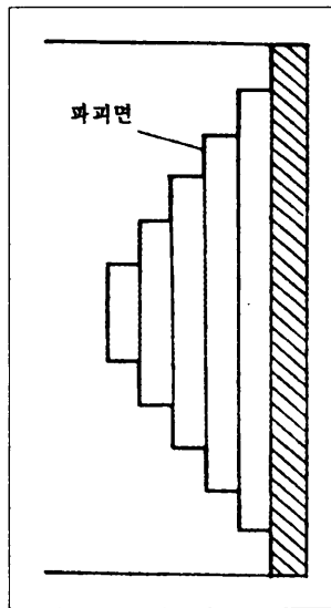
Fig. 16 Failure mechanism of cubic specimen
