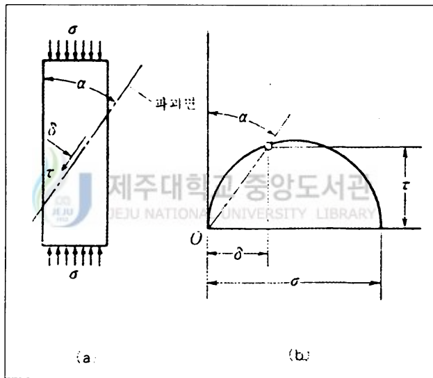
Fig. 4 Normal and shear stress at failure surface
