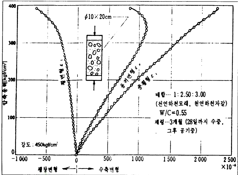
Fig. 1 Stress and strain relationship of concrete
