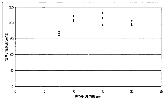
Fig. 17 Relationship of Compressive strength and specimen's diameter with H/D=2
