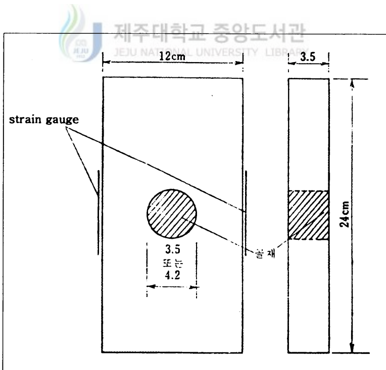
Fig. 6 Specimen to confirm Taylor-Broms theory
