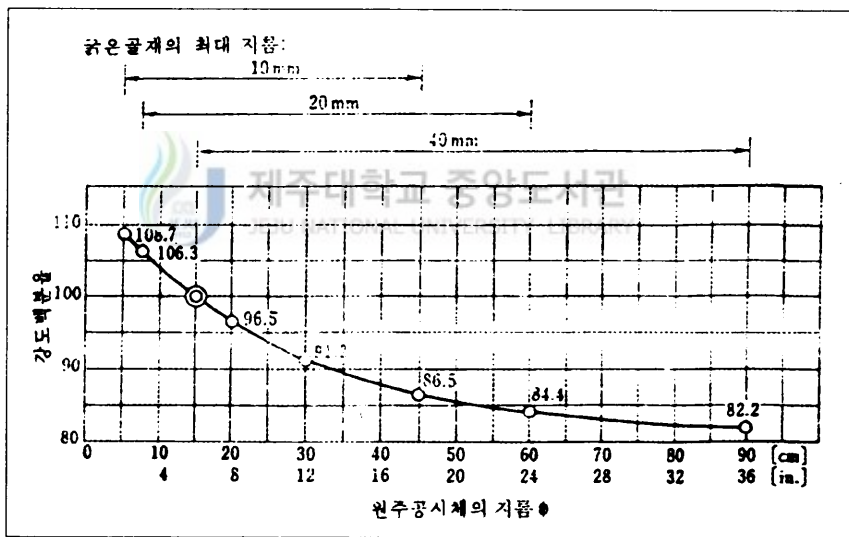
Fig. 14 Relationship of compressive strength and size of specimen
