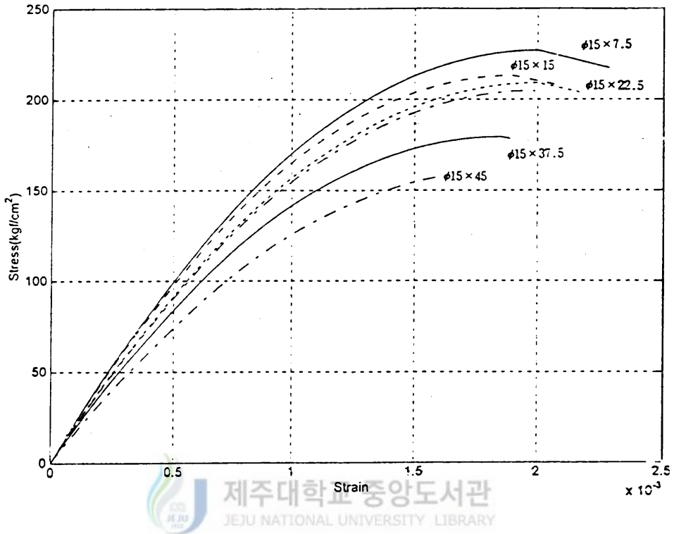
Fig.19 Stress-strain curve of cylinder specimens
