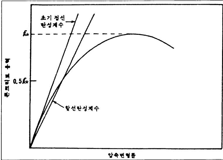
Fig. 3 Tangent modulus and secant modulus
