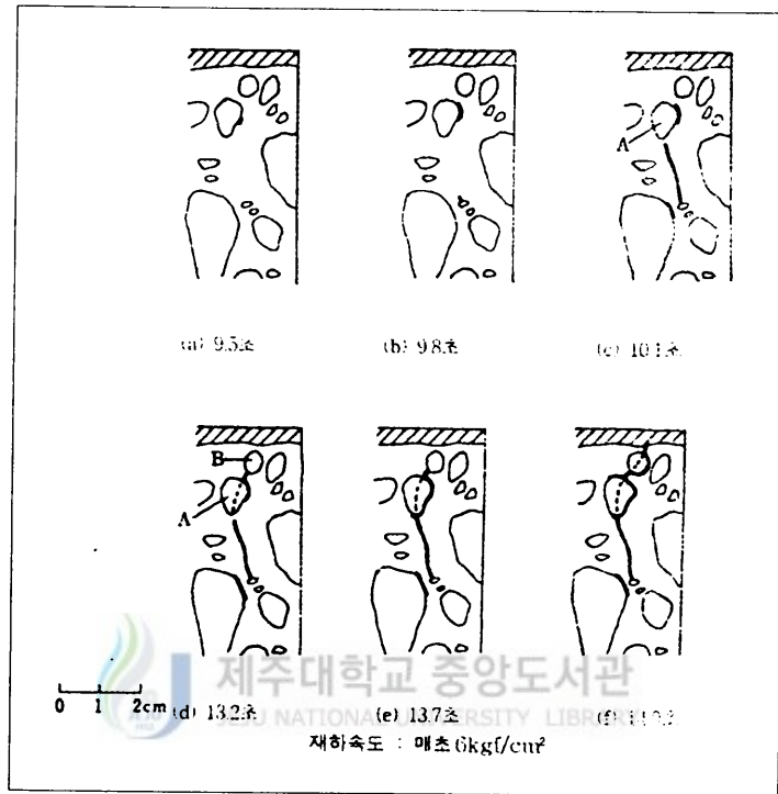
Fig. 12 Development of micro crack
