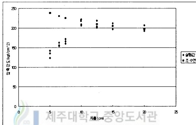
Fig.21 Comparison of this experimental and Cho's analytical results
