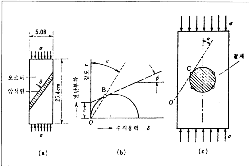
Fig. 5 Taylor-Broms theory on bond crack
