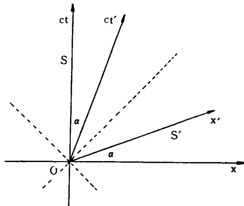
Figure 1. A Minkowski diagram in which two space dimensions are ignored. The angle is such that \tan \alpha = v/c , if v is the velocity of the frame S' relative to S .
