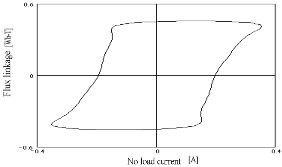
c) Hysteresis loop
