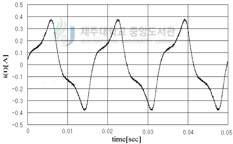
a) Measured current
