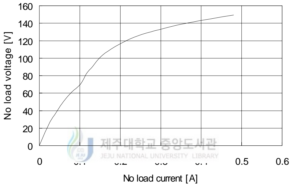
Fig. 2 RMS saturation characteristic of a single phase transformer
