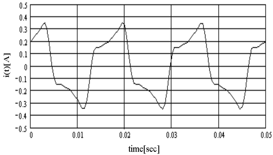
b) Computed current
