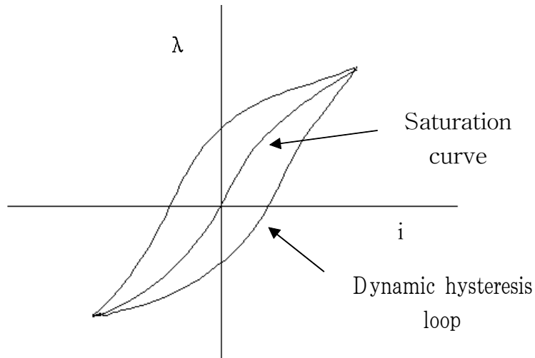
Fig. 1 Dynamic hysteresis loop and saturation curve
